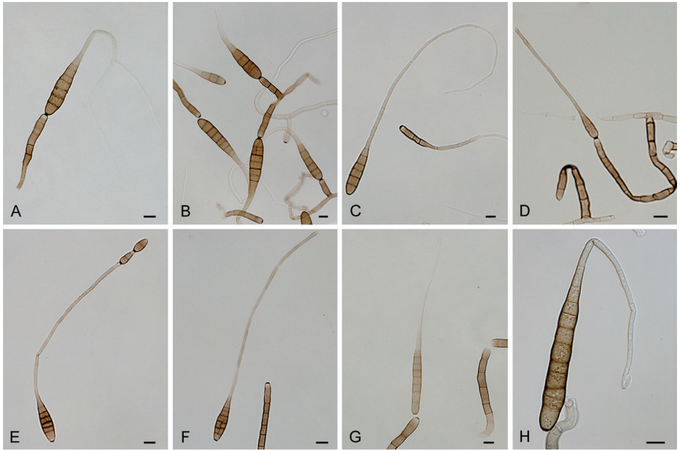
Fig. 19. Alternaria sect. Porri : conidia and conidiophores. A–C. A. daucii . D–F. A. pseudorostrata . G–H. A. solani . Scale bars = 10 \mu m.
