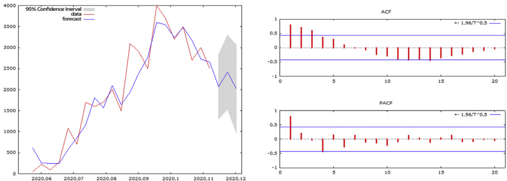
Fig. 2. Correlogram and ARIMA forecast graph for the 2019-nCoV incidence.
