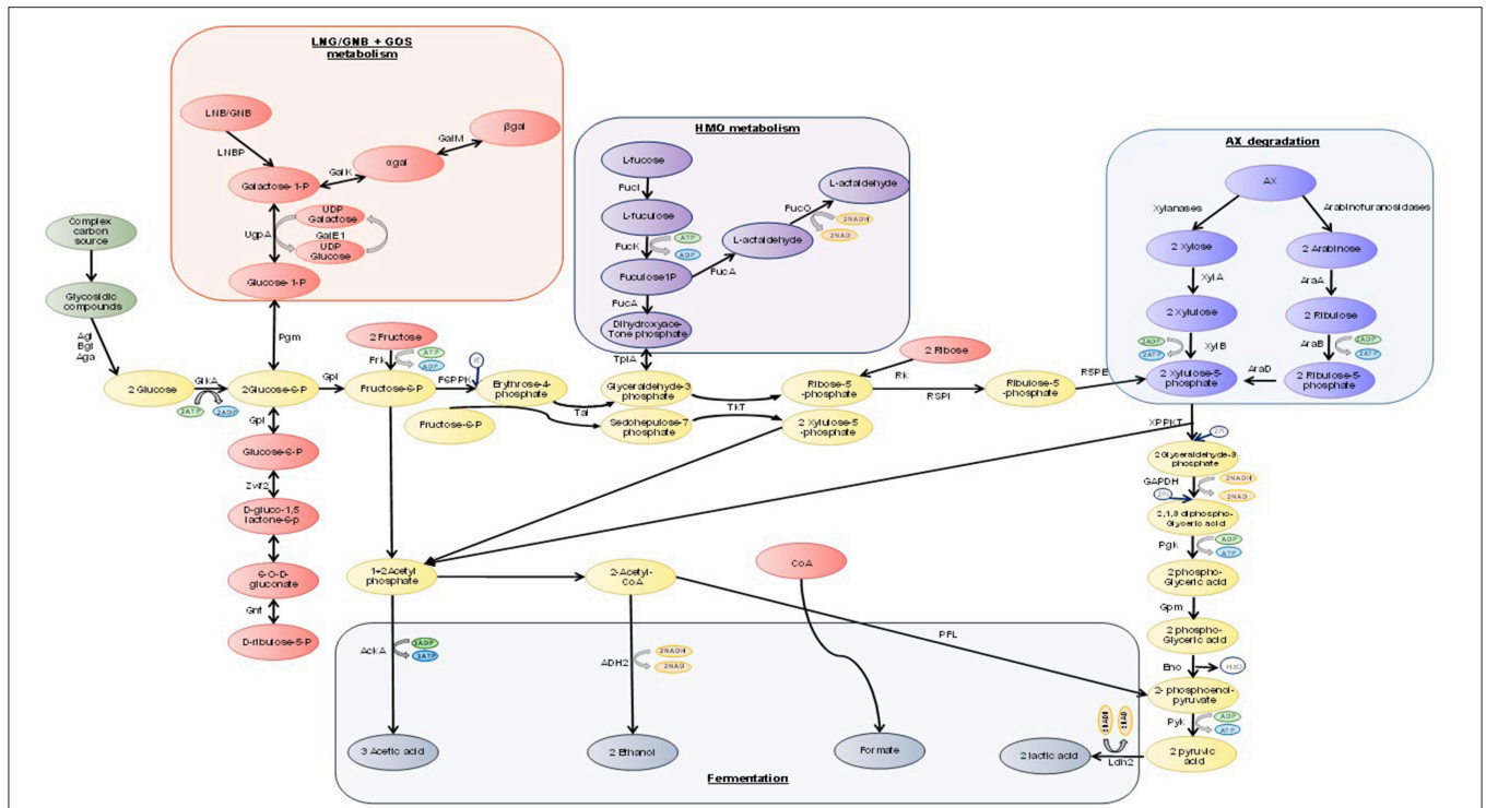
FIGURE 1 | A schematic representation of carbohydrate degradation through the “bifid shunt” in bifidobacteria. Abbreviations: AckA, acetate kinase; Adh2, Aldehyde-alcohol dehydrogenase 2; Aga, α-galactosidase; Agl, α-glucosidase; AraA, L-arabinose isomerase; AraB, Ribulokinase; AraD, L-ribulose-5-phosphate 4-epimerase; Bgl, β-glucosidase; Eno, enolase; GalE1, UDP-glucose 4-epimerase; GalK, galactokinase; GalM, galactose mutarotase; GAPDH, glyceraldehyde-3-phosphate dehydrogenase C; GlkA, glucokinase; Gnt, 6-phosphogluconate dehydrogenase; Gpi, glucose 6-phosphate isomerase; Gpm, phosphoglycerate mutase; Frk, fructokinase; F6PPK, fructose-6-phosphoketolase; Fucl, L-fucose isomerase; FucK, L-fuculose kinase; Fuca, L-fuculose-1-phosphate aldolase; FucO, lactaldehyde reductase; Ldh2, lactate dehydrogenase; LNBp, lacto-N-biose phosphorylase; Pggk, phosphoglyceric kinase; Pgm, phosphoglucomutase; Pfl, formate acetyltransferase; Pyk, pyruvate kinase; Rk, ribokinase; R5PI, ribose-5-phosphate isomerase; R5PE, ribulose-5-phosphate epimerase; Tal, transaldase; Tkt, transketolase; TpiA, triphosphate isomerase; UgpA, UTP-glucose-1-phosphate uridylyltransferase; XPPKT, xylulose-5-phosphate/fructose-6-phosphate phosphoketolase; XylA, xylulose isomerase; XylB, xylulose kinase; Zwf2, glucose-6-phosphate 1-dehydrogenase; Pi, phosphate (based on a figure from a previous review Pokusaeva et al., 2011a).
