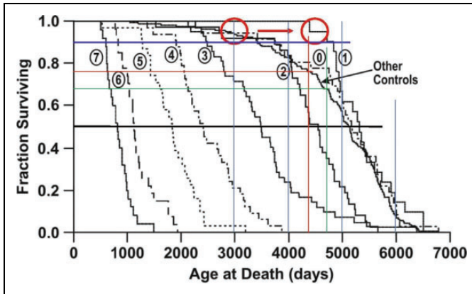
Figure 3. Fraction surviving curves of dogs with different lung burdens of inhaled plutonium-dioxide aerosols (Figure 4). 27 The red circles indicate that the shorter lived control dogs (5% mortality level) have a lifespan of about 3000 days, whereas the dogs in group 1 (initial plutonium lung burden of 0.16 kBq/kg) have a lifespan of about 4500 days, 50% longer. Also shown are the 10% and 50% mortality levels.
