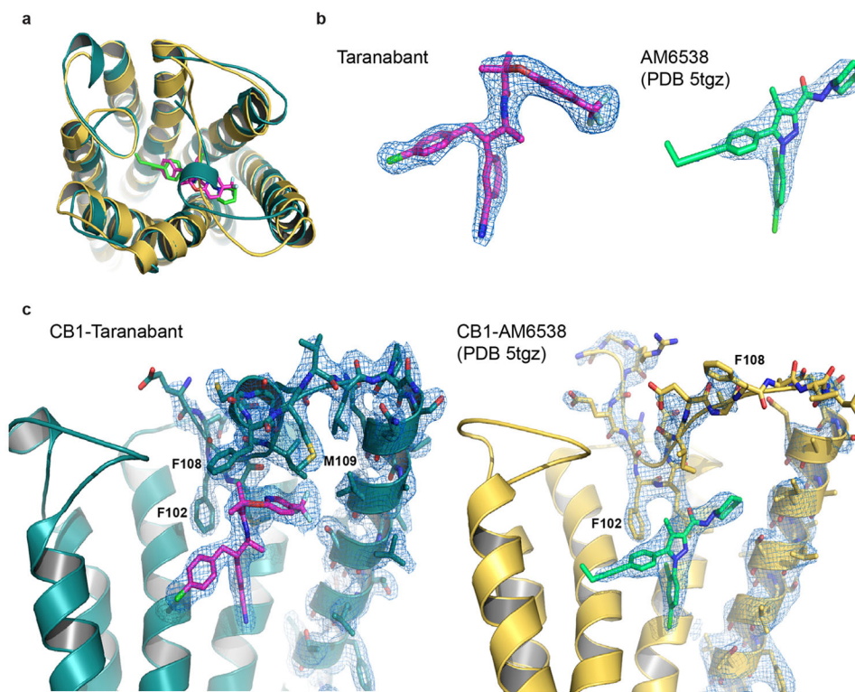
Extended Data Figure 9. Comparison of the structures of CB1 bound to taranabant and CB1 bound to AM6538 (ref. 34, PDB 5tgz)
