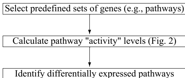
Figure 1 Outline of pathway level analysis of gene expression.
