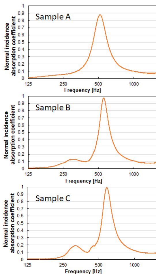
Figure 3. Results of the preliminary tests of Samples A, B, and C using an impedance tube (transfer function method). Tests were performed with a square impedance tube of 100 mm length; therefore, the upper limit of the measurement frequency was 1600 Hz.
