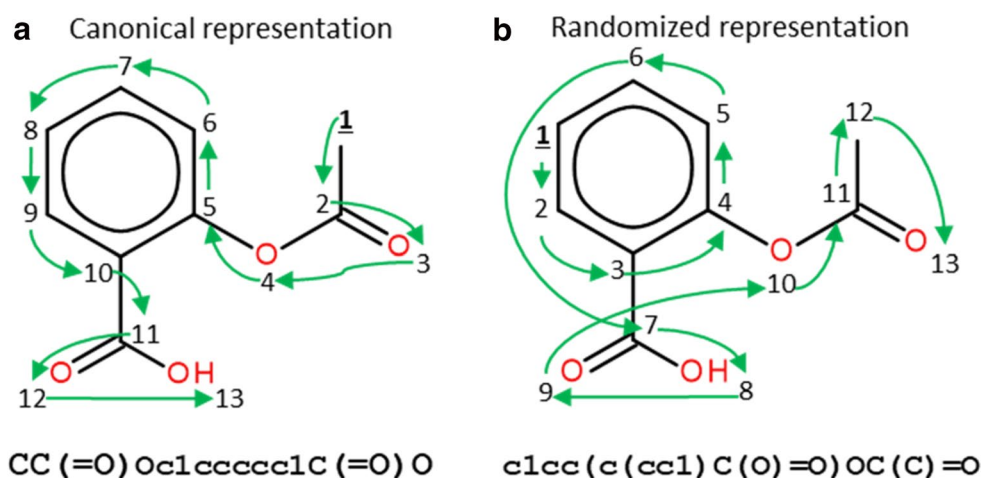
Fig. 4 Canonical (a) and randomized (b) SMILES representations of aspirin. Randomized SMILES correspond to the various representations of a molecule obtained by randomly selecting the starting node in the graph traversal algorithm, thus changing the order of the nodes traversed in the molecular graph (still using depth-first search). Numbers represent the order of graph traversal, where 1 is the initial node (user defined). Considering a as being the canonical representation of aspirin, b shows a different ordering of the atoms of the molecule. The final SMILES is one possible SMILES among all the randomized SMILES which can be generated. Green arrows indicate how the molecular graph is traversed. Both SMILES strings shown represent the same molecule but, as the atom numberings are different, the generated SMILES strings are, too. The original figure can be found in [47]
