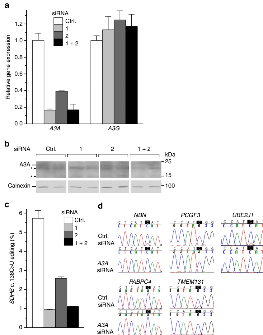
Figure 6 | Knockdown of APOBEC3A (A3A) reduces C>U RNA editing in M1 macrophages (a) A3A and APOBEC3G (A3G) gene expression in M1 macrophages that were transfected with a nonspecific ( Ctrl. ) or either one (1, 2) or equimolar mix (1 + 2) of two A3A-specific siRNAs at 100 nM concentration. Gene expression measurements are normalized to that for ACTB . (b) Immunoblot for A3A protein (23 kDa) of whole-cell lysates (10 \mu g protein) of two of each set of three replicate transfectants. Nonspecific signals are indicated by an asterisk (*). The signal for calnexin, a house-keeping protein, indicates total protein. (c) SDHB c.136C>U RNA-editing levels in the siRNA transfectants, which are determined by RT-qPCR. (d) Sanger sequence chromatogram traces of amplified cDNA fragments, indicating reduced site-specific RNA editing for five other genes in A3A-specific siRNA 1 compared with Ctrl. transfectants. Mean and range ( n = 3 ) are shown for a and c .
