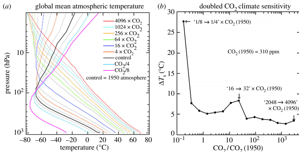
Figure 7. (a) The calculated global mean temperature for successive doublings of CO 2 (legend identifies every other case) and (b) the resulting climate sensitivity (1 × CO 2 = 310 ppm).
