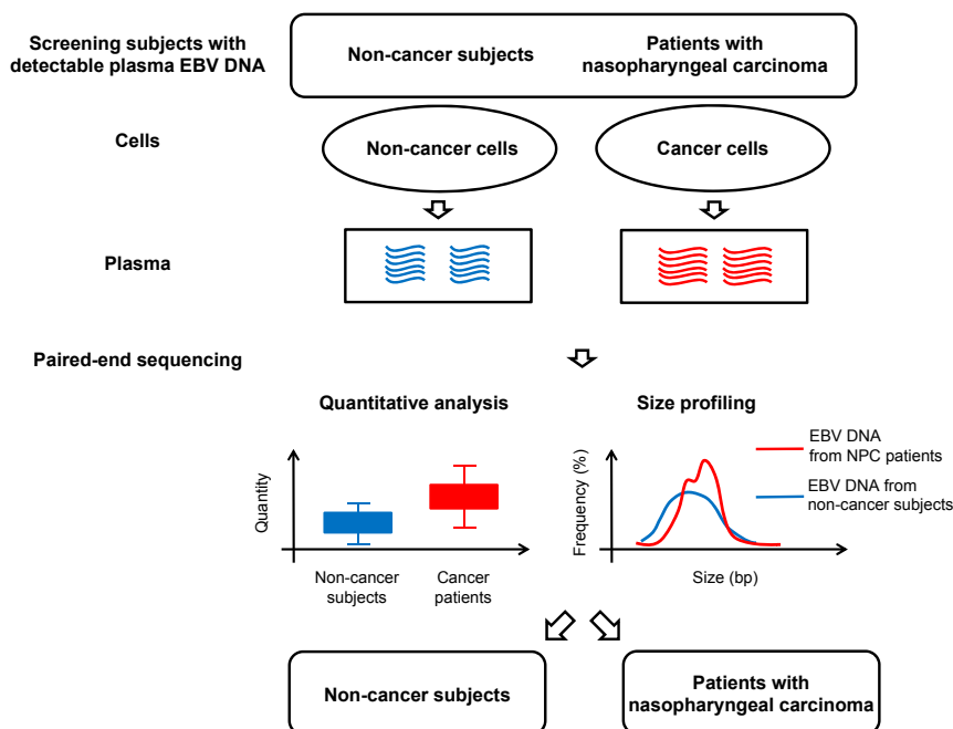
Fig. 1. Quantitative and size profile analysis of plasma EBV DNA in patients with nasopharyngeal carcinoma (NPC) and non-NPC subjects.
