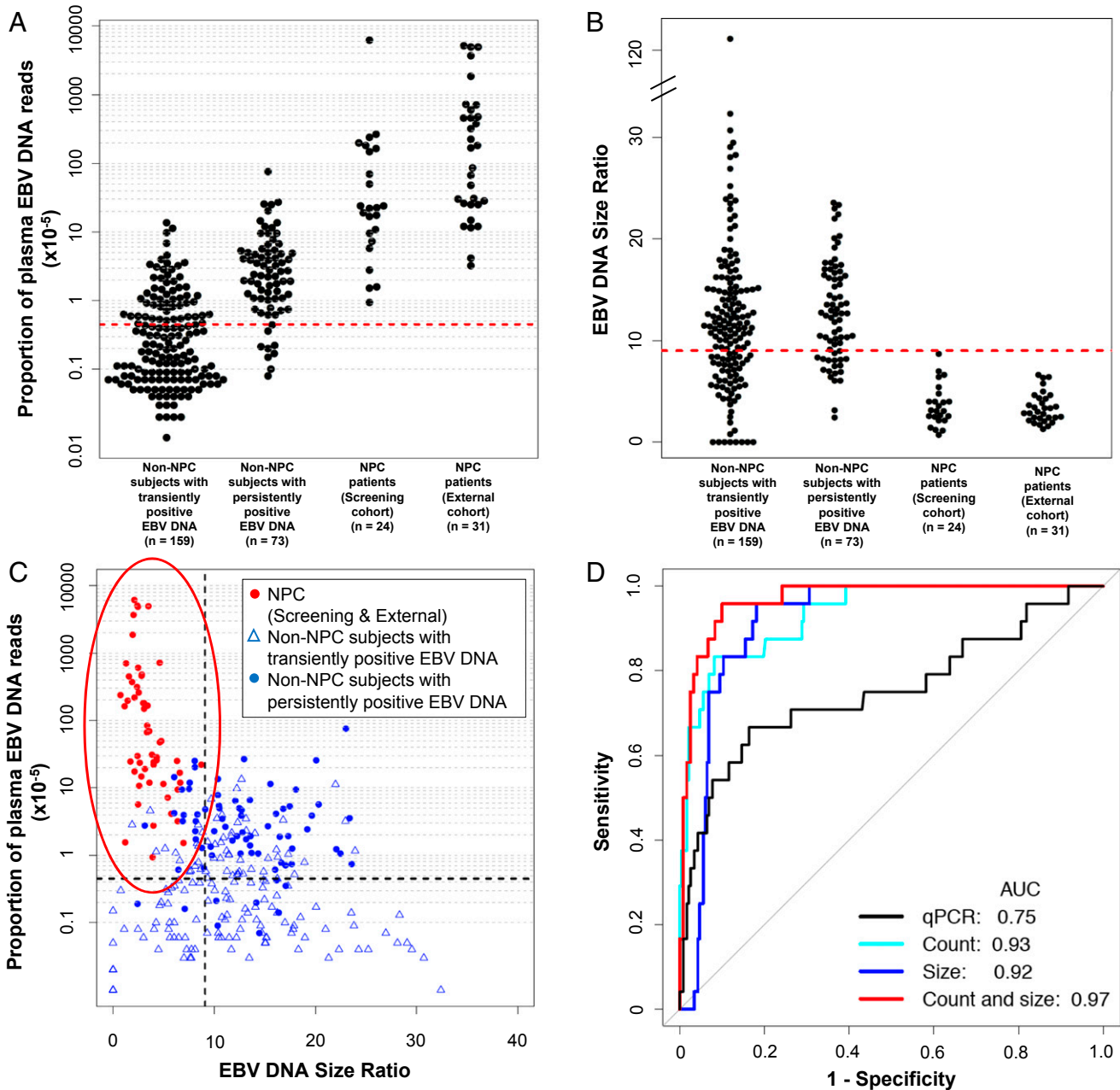
Fig. 5. Count- and size-based analyses of plasma EBV DNA by target-capture sequencing in the validation sample set. (A) The proportions of plasma EBV DNA reads of the NPC patients and non-NPC subjects are shown. The same cutoff value of 4.5 \times 10^{-6} defined in exploratory dataset is denoted by the red dotted line. (B) The EBV DNA size ratios of the NPC patients and non-NPC subjects are shown. The same cutoff value of 9.1 defined in the exploratory dataset is denoted by the red dotted line. (C) Plot of the proportions of plasma EBV reads and corresponding size ratio values for all of the cases in the validation sample set. The same cutoff values in the count- and size-based analyses defined in the exploratory sample set are denoted by the gray dotted lines. The red oval highlights the quadrant with cases that passed the cutoffs in the combined count- and size-based analysis. (D) ROC curves for the count-based analysis, size-based analysis, combined sequencing analysis, and real-time PCR analysis are shown. Area under the curve (AUC) values are shown.
