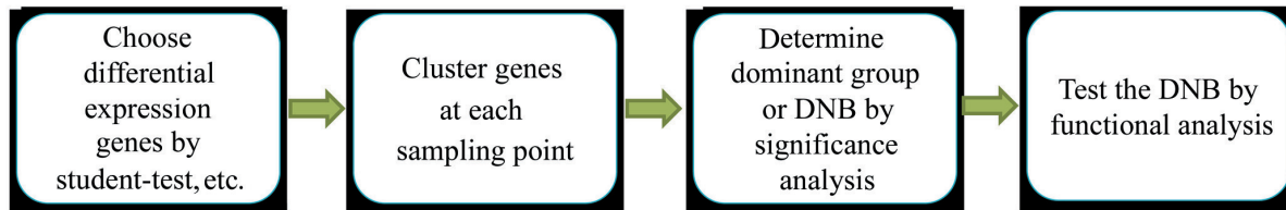
Figure S6: | Flowchart of the algorithm.
