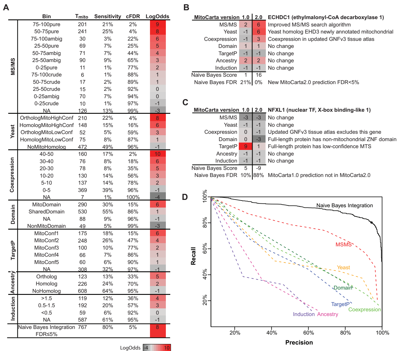
Figure 2. Naïve Bayes integration improves accuracy over individual data sources. (A) Accuracy of each of seven data sources and the Maestro naïve Bayes integration, calculated from the human T_{mito} and T_{non-mito} genes. (B) LogOdds scores for gene ECHDC1 , in MitoCarta2.0 but not MitoCarta1.0, highlights improvements in three data sources (C) LogOdds scores for gene NFXL1 , in MitoCarta1.0 but not MitoCarta2.0, highlights improvements to RefSeq gene models—as previous 58aa protein fragment XP.001052092 has been replaced with 918aa full-length protein NP.598682. (D) ROC curve shows accuracy of each data source individually as well as the combined naïve Bayes Integration. Black circle indicates 5% FDR threshold.
