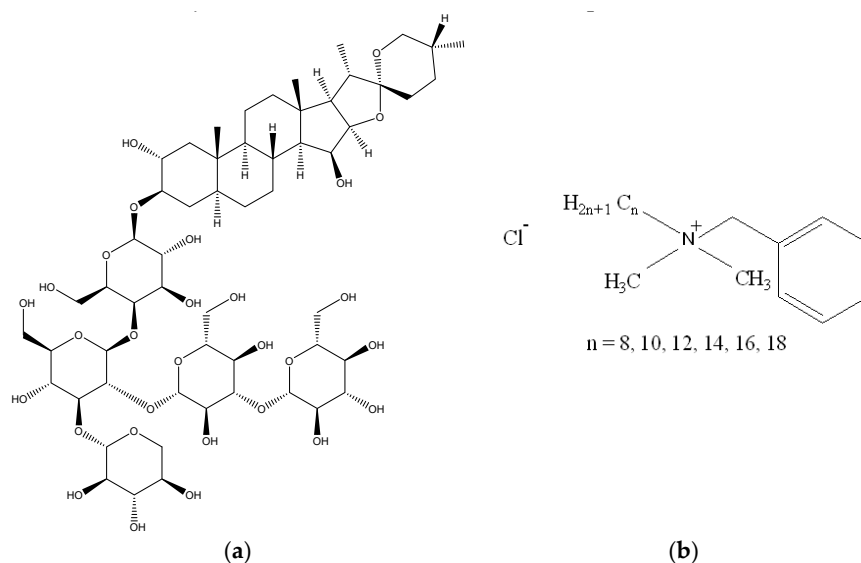
Figure 12. Structures of digonin (a) and benzalkonium chloride (b).
