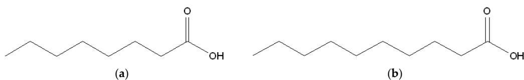
Figure 15. Structures of caprylic acid (a) and capric acid (b).
