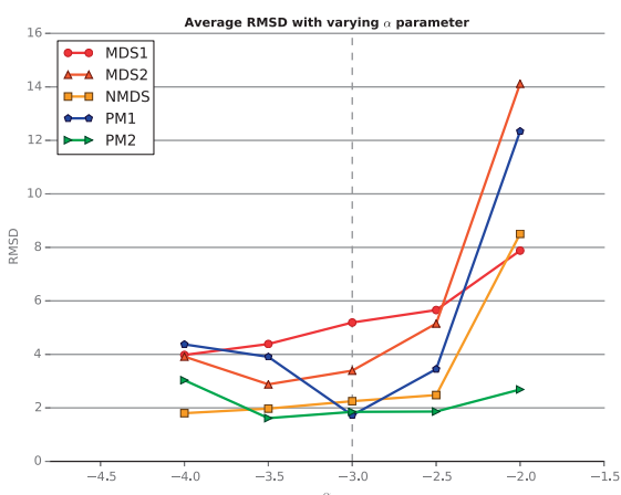
Fig. 2. Performance evaluation for simulated data, varying the parameter \alpha . The figure plots the average RMSD of the inferred structures for a range of \alpha values. As \alpha increases, the SNR of the dataset also increases
