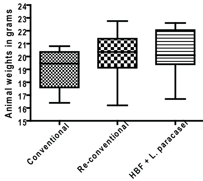
Box-and-whisker plots
