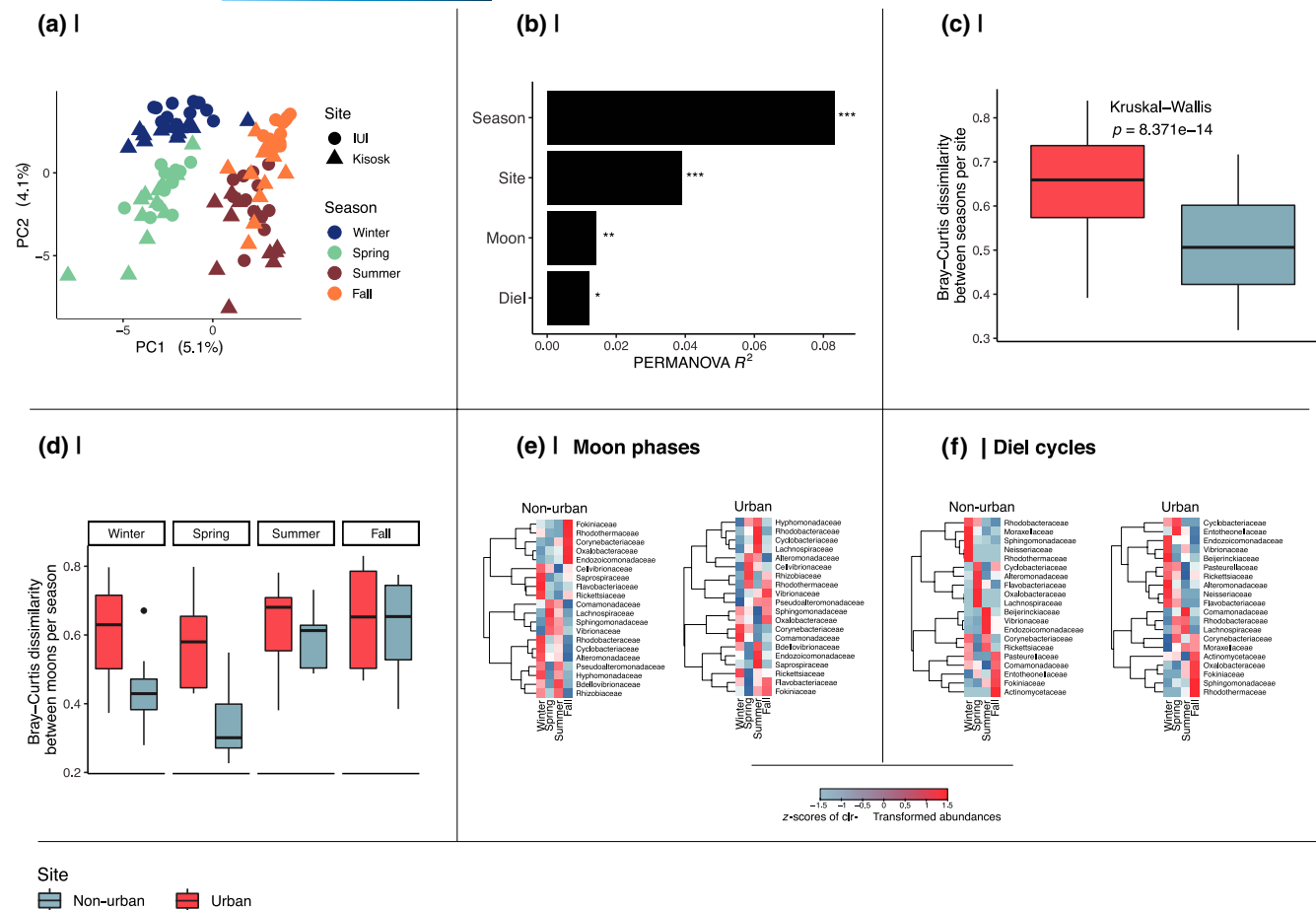
FIGURE 5 Coral microbiome activity changes over diel cycles and moon phases. (a) Principal component analysis (PCA) of bacterial communities over seasons and areas. PCA is based on CLR-transformed amplicon sequence variant (ASV) abundances using Euclidean distances. (b) Overall factors that influence the bacterial community composition denoted by PERMANOVA R^2 values. Significance values indicate *p \leq .05 , **p \leq .01 , and ***p \leq .001 . (c) Seasonal bacterial community dissimilarities between urban and non-urban areas. (d) Community dissimilarities between new and full moons per season and area. Dissimilarities were calculated as Bray Curtis distances. Differentially abundant ASVs clustered by family for (e) moon phases and (f) diel cycles. ASV counts were binned into families and transformed using the CLR transformation. Z-scores were applied on families across seasons (rows), and hierarchical clustering was done using the “complete” method
