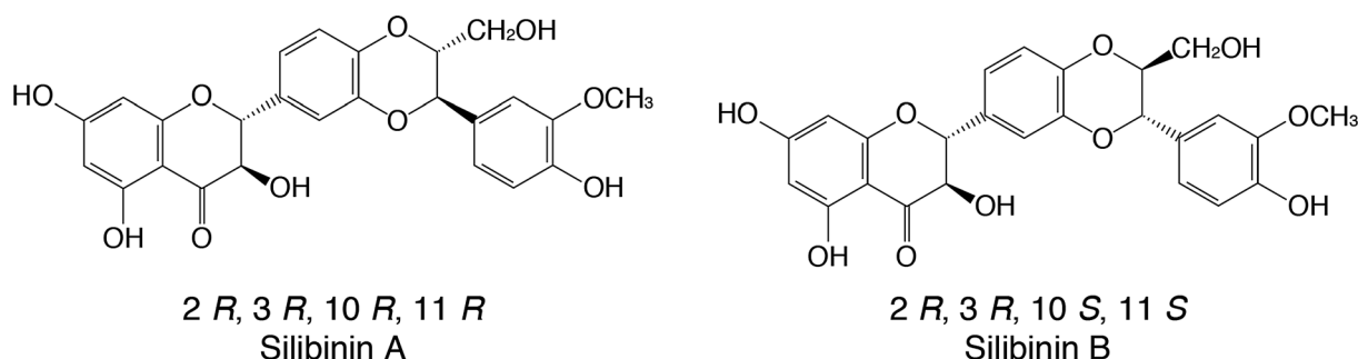
Fig. 1 Chemical structure of the silibinin diastereoisomers, silibinin A and silibinin B ( C_{25}H_{21}O_{10} )
