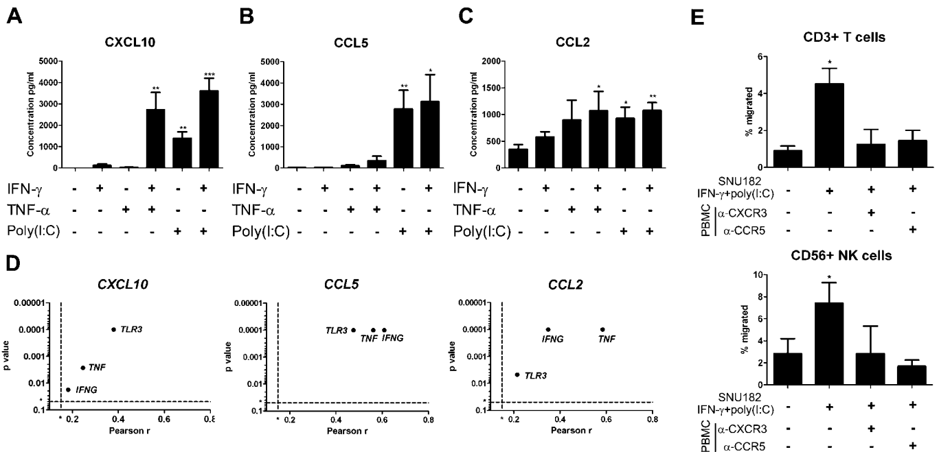
Figure 5 The production of CXCL10, CCL5 and CCL2 by HCC cell lines is induced by interferon \gamma ( \text{IFN}\gamma ), tumour necrosis factor \alpha ( \text{TNF}\alpha ) and Toll-like receptor 3 (TLR3) ligands. ELISA for (A) CXCL10, (B) CCL5 and (C) CCL2 concentration in culture supernatants from the SNU-182 hepatocellular carcinoma (HCC) cell line 24 h after stimulation with \text{IFN}\gamma , \text{TNF}\alpha and/or poly(I:C). Two-tailed Student unpaired t test; * p < 0.05 ; ** p < 0.01 ; *** p < 0.001 compared with unstimulated control. Graphs show the means and SD from three independent experiments. (D) CXCL10, CCL5 and CCL2 RNA are positively correlated with IFNG, TNF and TLR3 in patients with HCC (training and validation cohort, n = 172 ). Graphs show the p value against Pearson correlation coefficients r . Dotted lines show limits of significance for r ( r = 0.15 ) and p ( p = 0.05 ). (E) Transmigration assay with peripheral blood mononuclear cells (PBMCs) isolated from healthy donors ( n = 3 ) towards unstimulated or stimulated SNU-182 cells with \text{IFN}\gamma and poly(I:C) 24 h prior to transmigration. In blocking experiments, PBMCs were pretreated with anti-CXCR3 or anti-CCR5 neutralising antibodies at 37^\circ\text{C} for 1.5 h. Graphs show means and SEM. p Values were calculated using paired t test against basal transmigration towards unstimulated HCC. * p < 0.05 . NK, natural killer.
